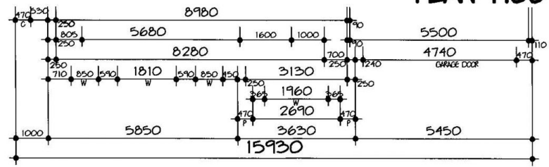
GROUND FLOOR PLAN 1:100
